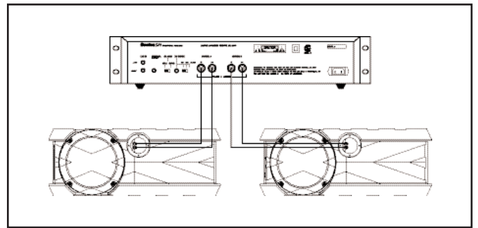
Connecting two Voyager Sub12 subwoofers to the SA1
